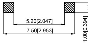
PCB WELDING DRAWING PCB 焊接图
