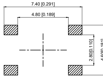
PCB. Welding board PCB.焊接板
