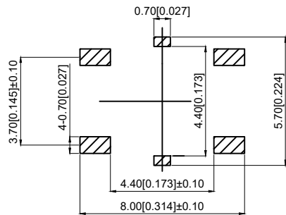
PCB. Welding board PCB.焊接板
