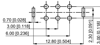
PCB LAYOUT BOTTOM VIEW PCB布局底视图
