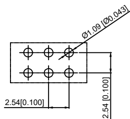
PCB WELEING DRAWING
