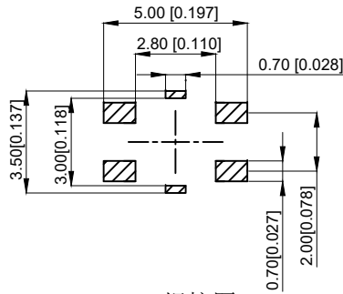
PCB.焊接图 PCB.WELDING DRAWING
