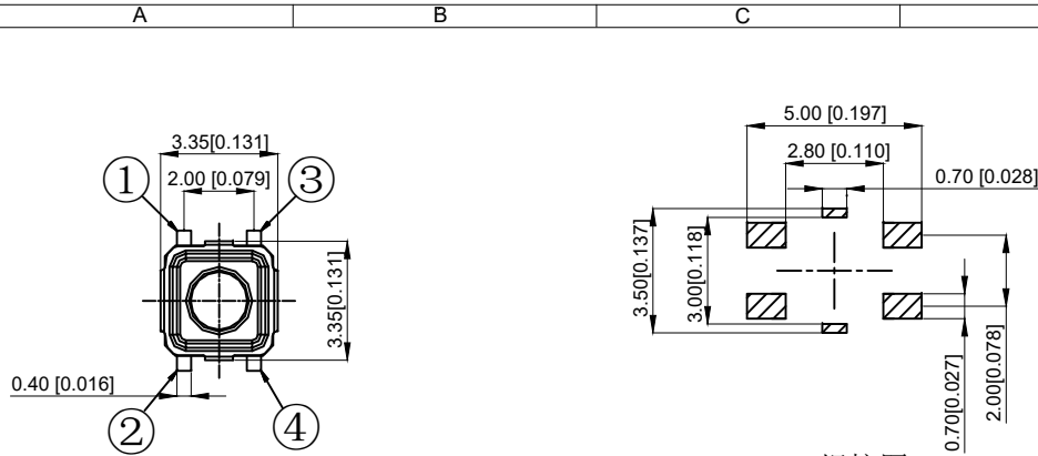
PCB.焊接图 PCB.WELDING DRAWING
