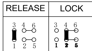
CIRCUIT DIANGRAN
