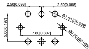
PCB board welding dimension drawing PCB板焊接尺寸图
