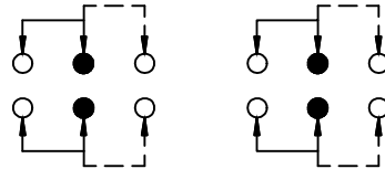
SCHMATIC(SHORTING)
