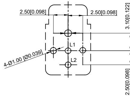
PCB.Welding diagram PCB.焊接图
