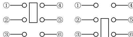
Circuit diagram Normal: 1-2 on 4-5 on Press: 2-3 on 5-6 on
